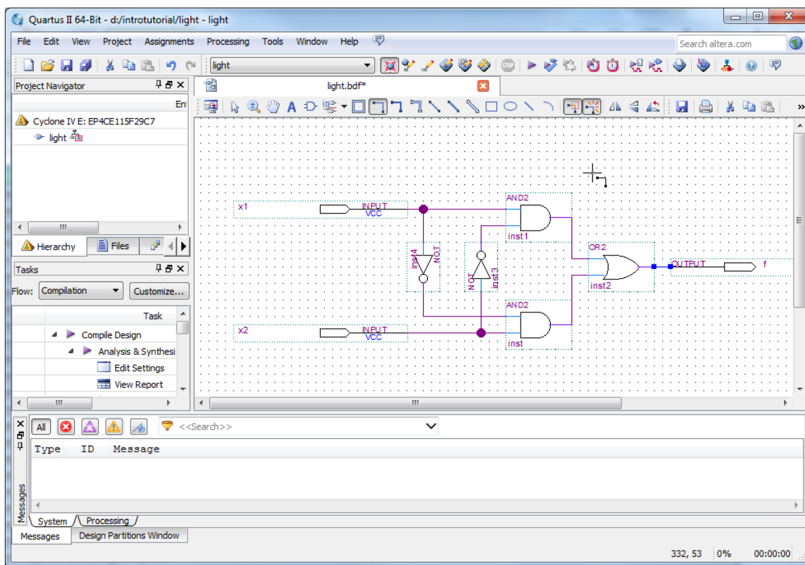
Figure 20. The completed schematic diagram.
