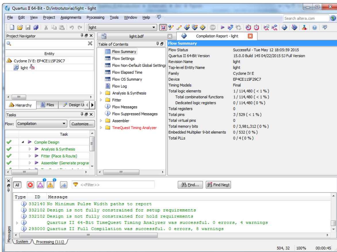
Figure 21. Display after a successful compilation.
