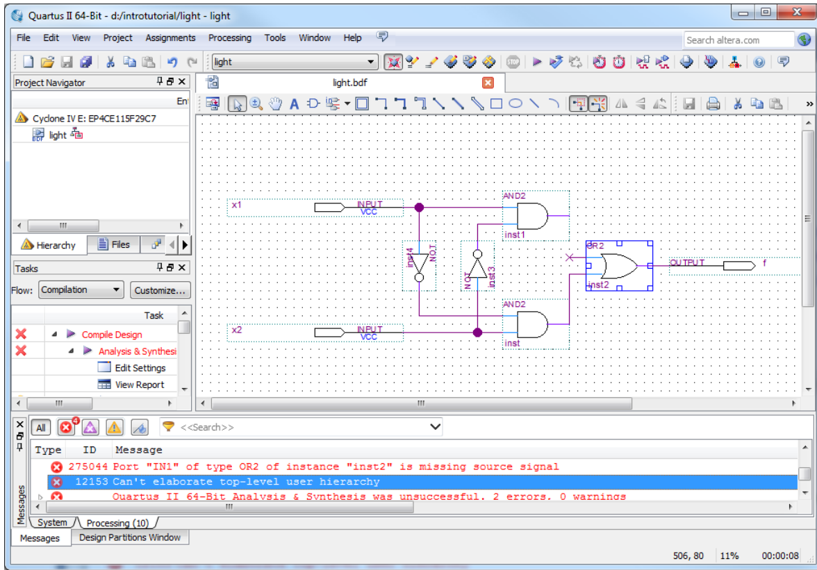
Figure 24. Identifying the location of the error.
