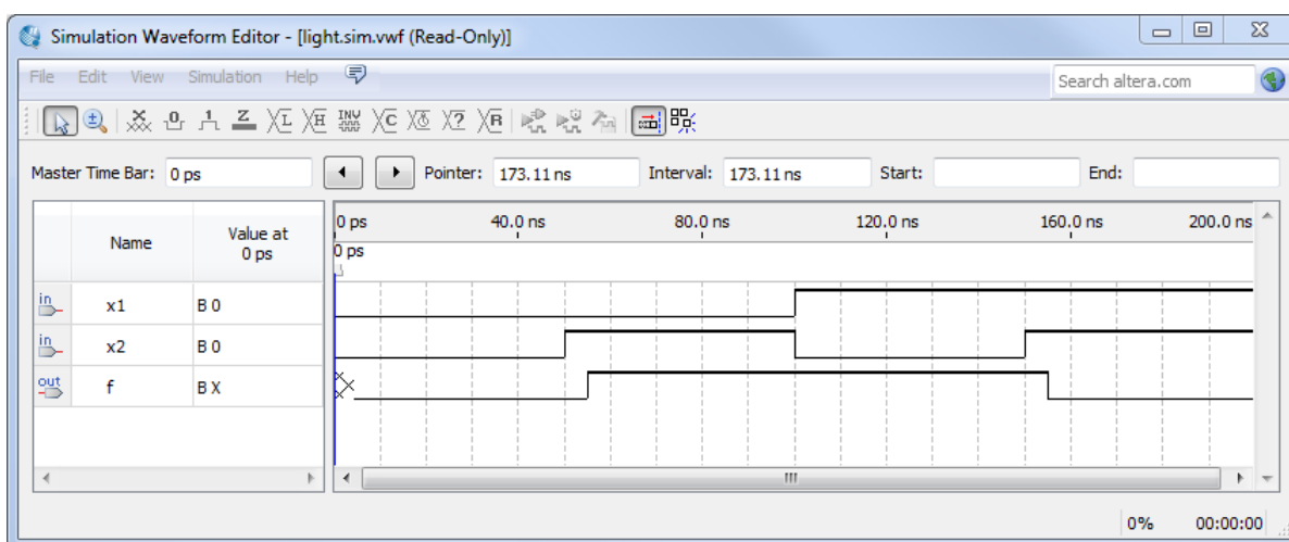
Figure 38. The result of timing simulation.
