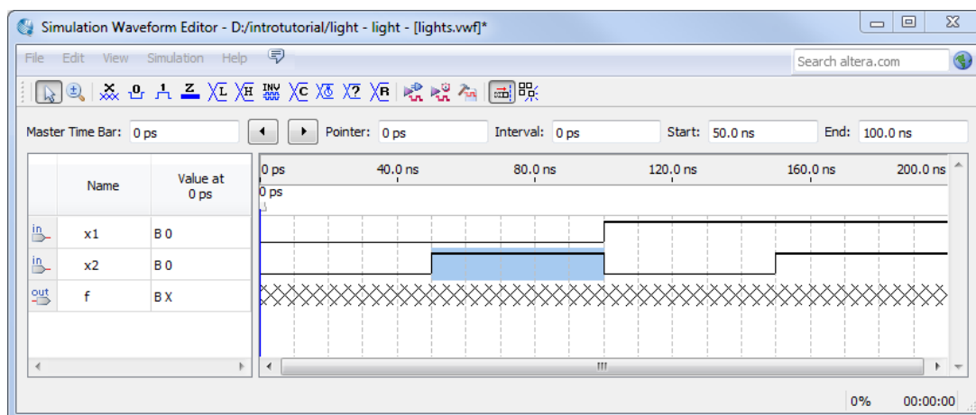
Figure 36. Setting of test values.
