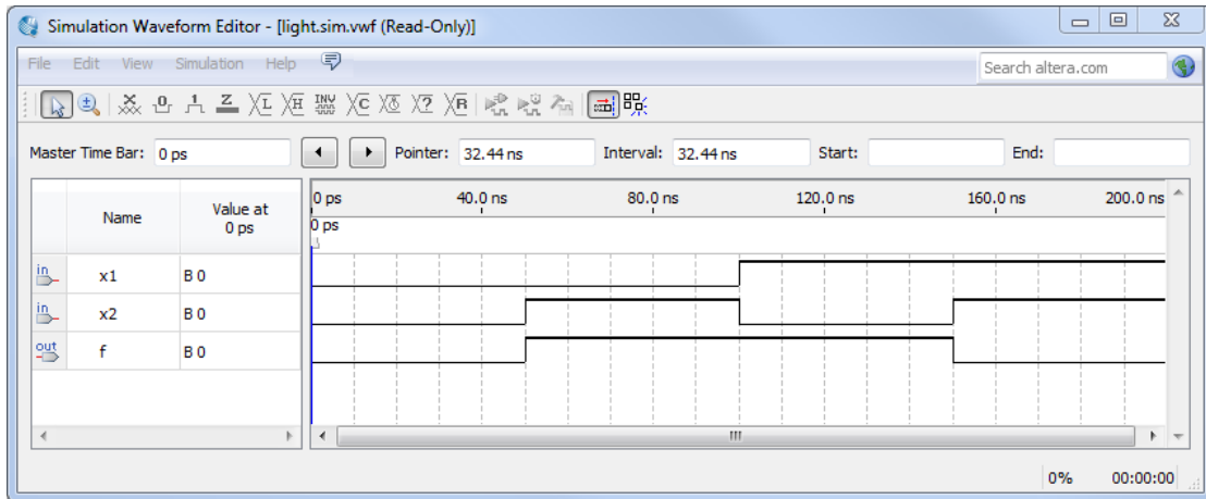
Figure 37. The result of functional simulation.
