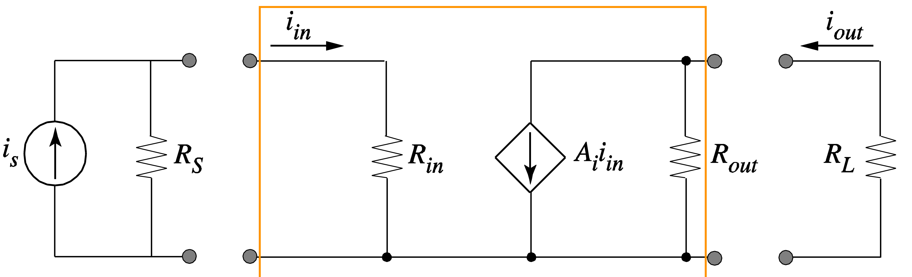
(b) Current Amplifier Model
