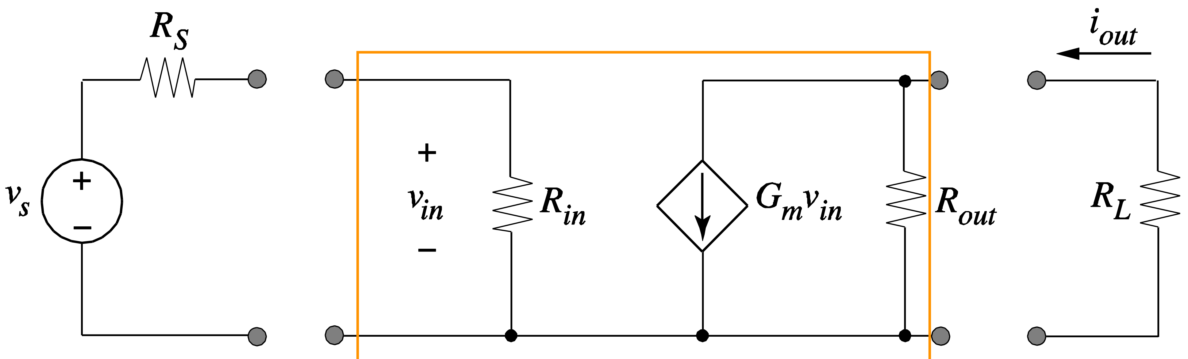
(c) Transconductance Amplifier Model
