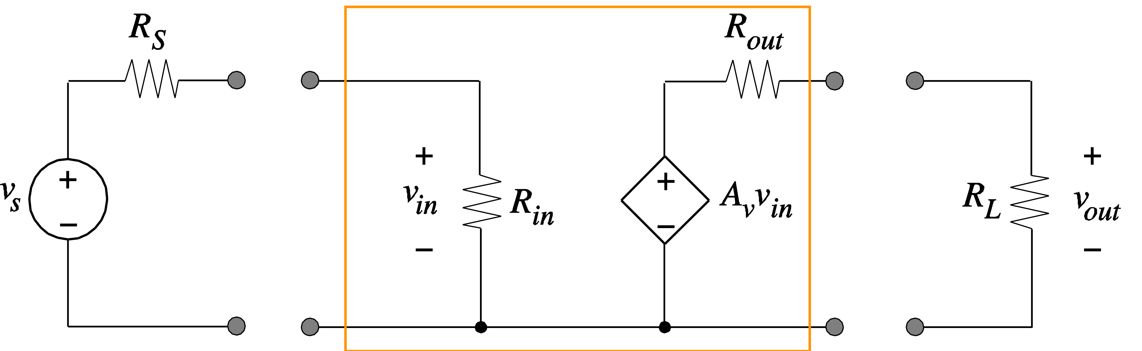
(a) Voltage Amplifier Model
