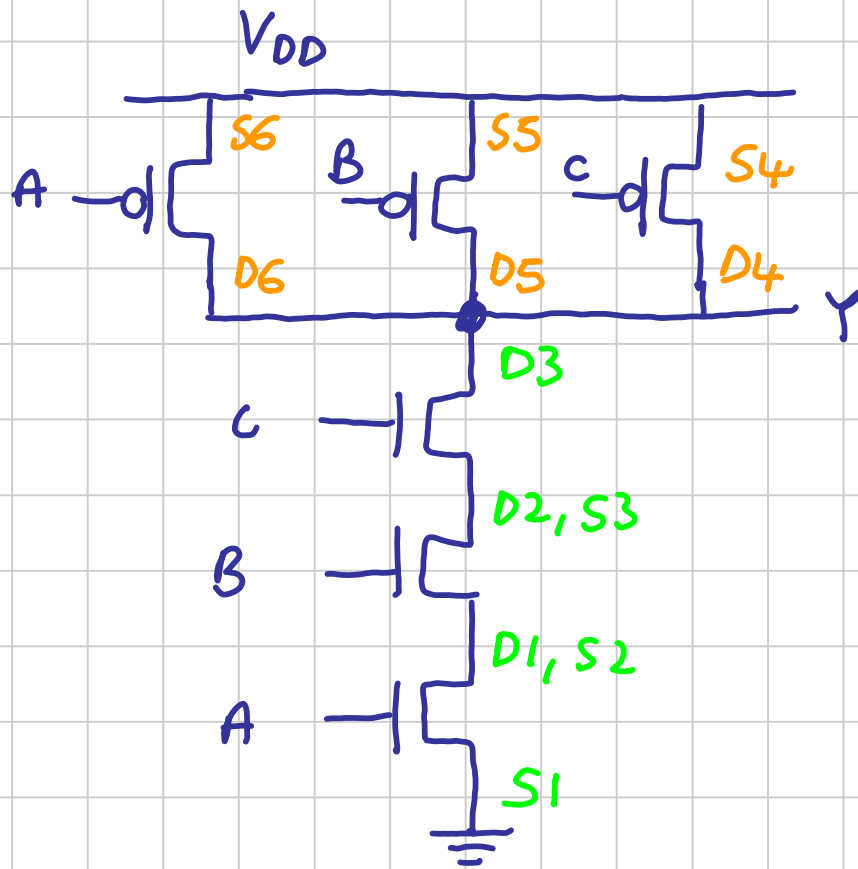
3-input NAND gate
