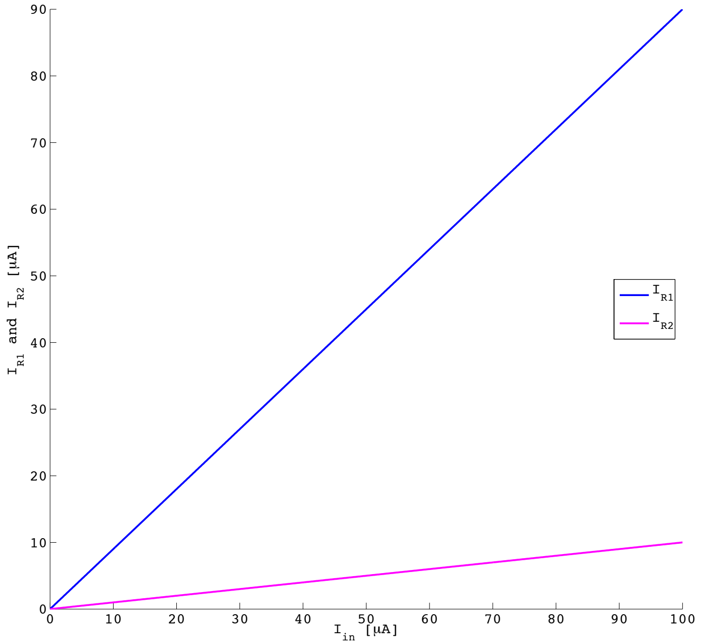
I_{R1} and I_{R2} vs. I_{in}
